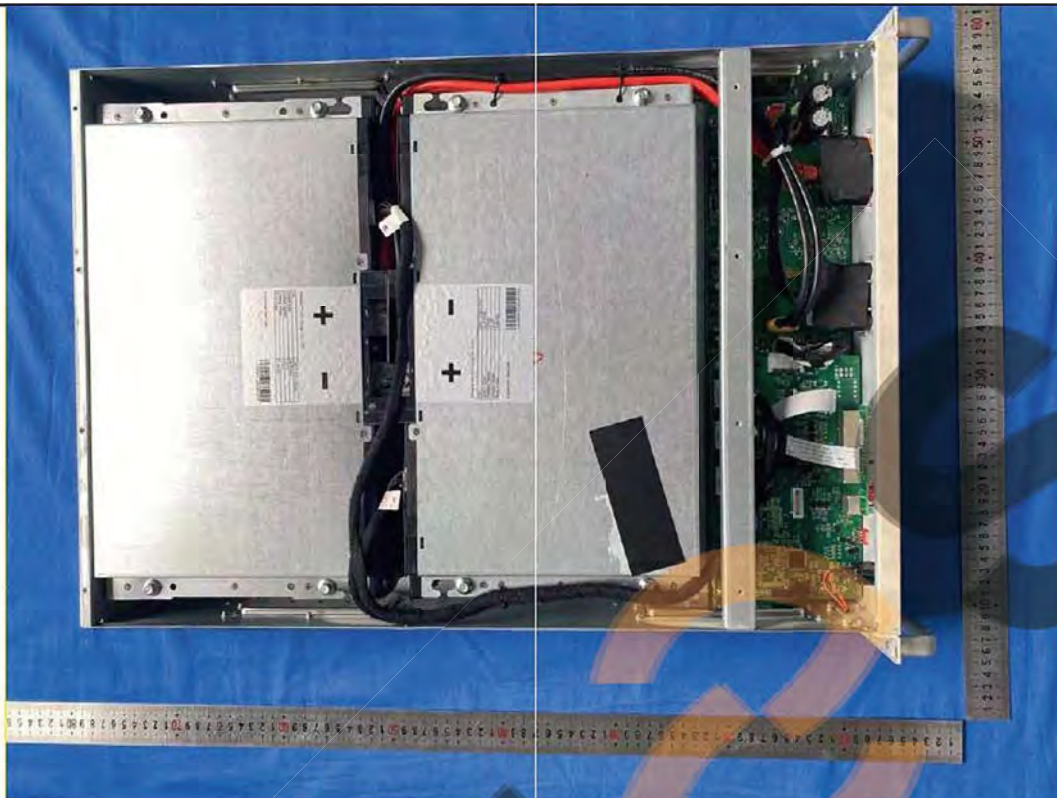
Figure 2b. Internal view of battery module
